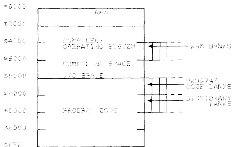
FIGURE 1 - MEMORY ORGANIZATION
